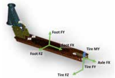
Fig. 4 - FEA Unit Loads
