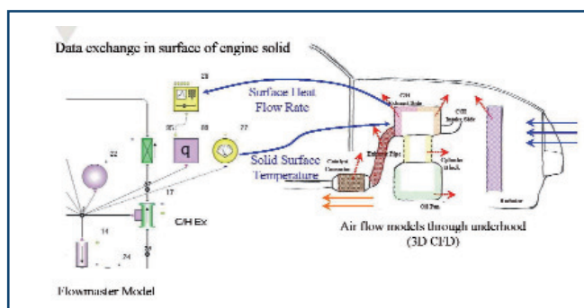
Full vehicle thermal management
